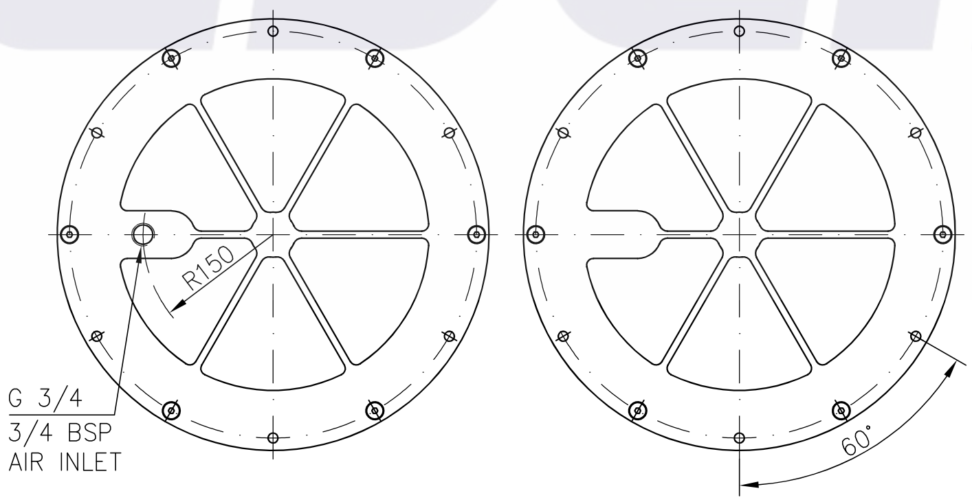
TOP VIEW (1:2)
