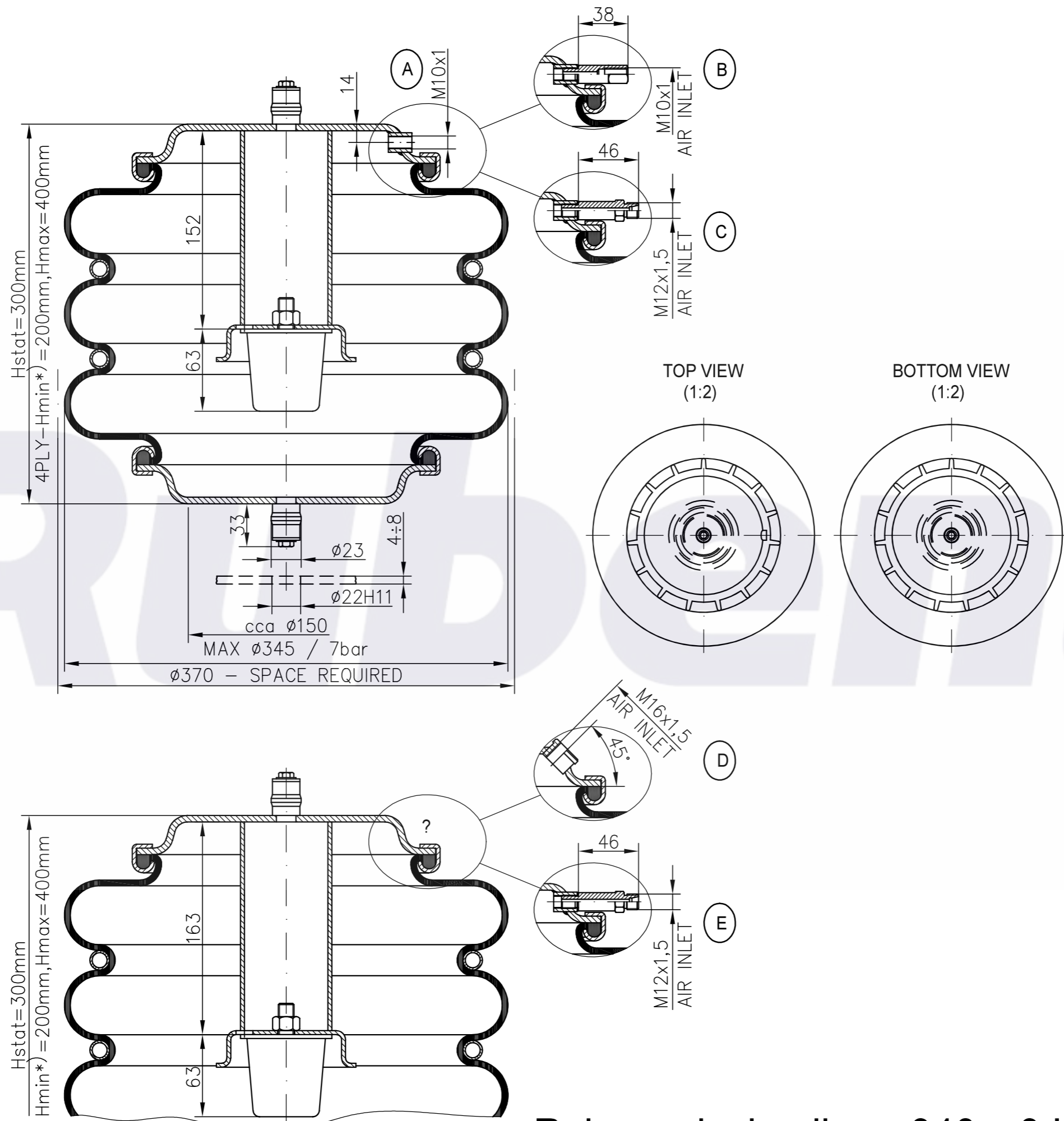
Rubena design line - 340 x 3 Karosa Recreo Crimp
