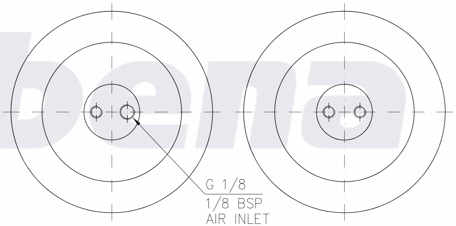
TOP VIEW
