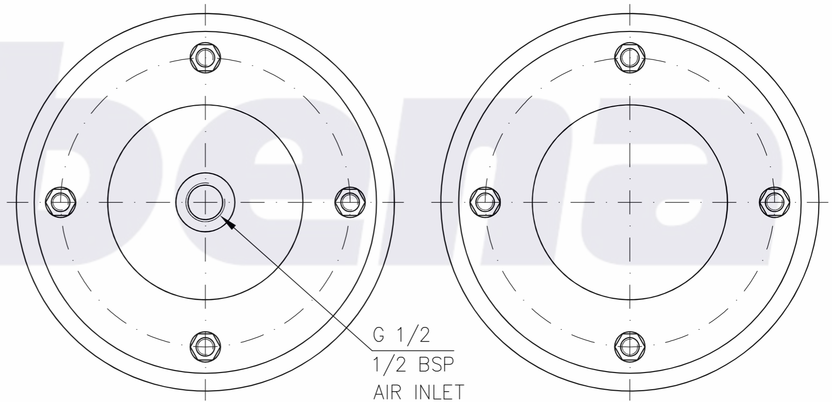
TOP VIEW
